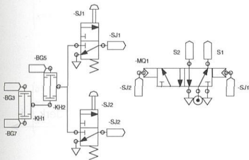
Figure 13. Memory implementation in a pure pneumatic system.
