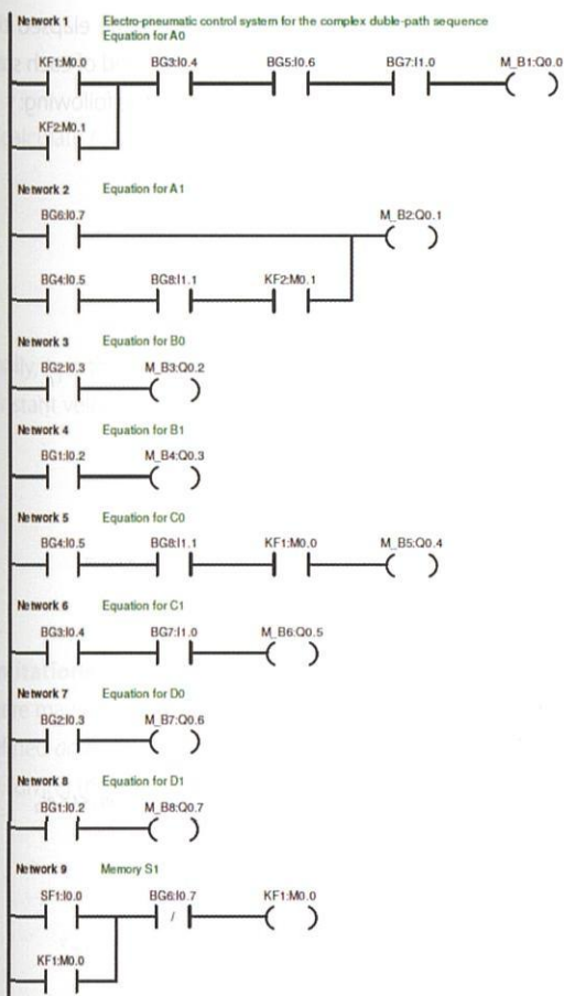
Figure 14. Digital control of an electro-pneumatic system.
