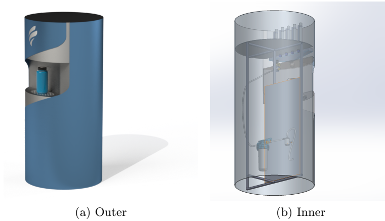
Fig. 1. BiboLink: structure design.
