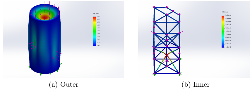
Fig. 5. Structure: stress simulation results.
