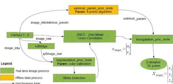
Figure 9. Vision target detection implementation.
