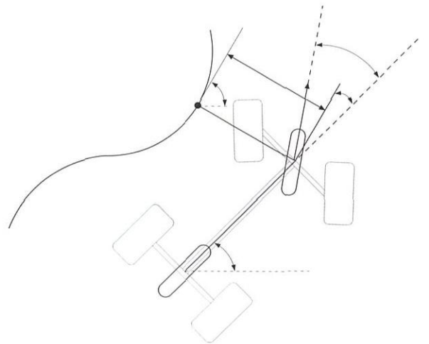
Figure 6. Path tracking.
