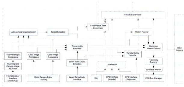
Figure 4. Software architecture.
