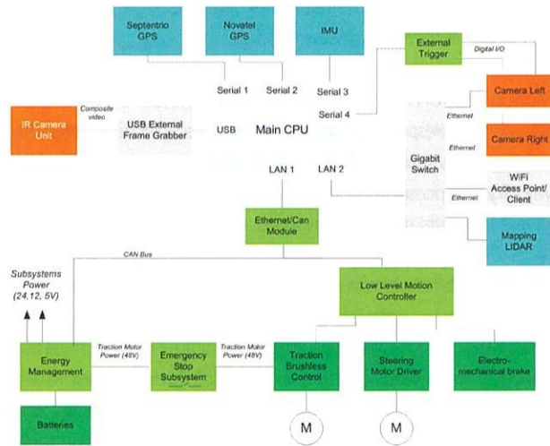
Figure 3. System architecture.
