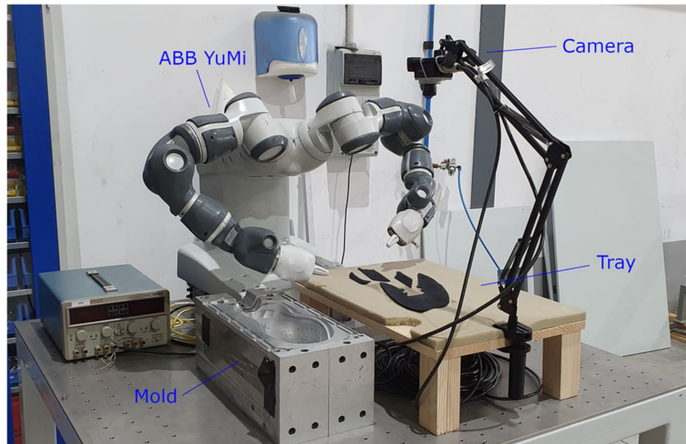
Fig. 3 Proposed system with an ABB YuMi robot, camera, shoe mold and tray [14]
