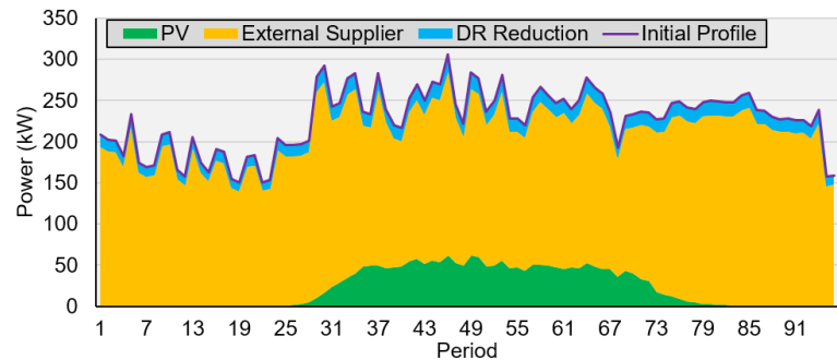
Fig. 6. Scheduling results for all the resources of the community.
