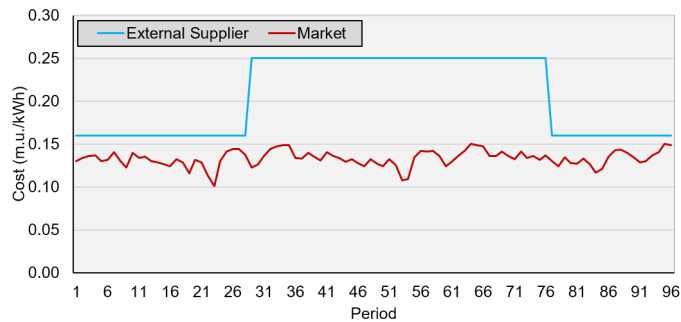
Fig. 4. Electricity prices during the case study.
