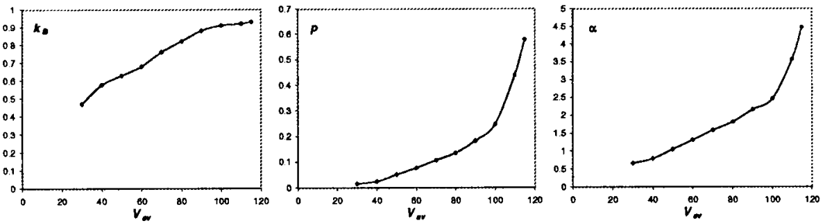
Figure 8: Gain k_B , pole p and fractional order \alpha versus v_{av} for \Delta v = 20 \text{ km h}^{-1} , n_l = 2 , l = 1000 \text{ m} and \phi_1(t; 0) \in [1, 8] \text{ vehicles s}^{-1} .
