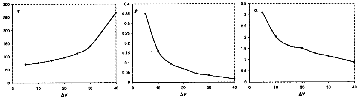
Figure 4: Time delay \tau , pole p and fractional order \alpha versus \Delta v for v_{av} = 50 \text{ km h}^{-1} , n_l = 1 , l = 1000 \text{ m} , \phi_1(t; 0) \in [1, 8] \text{ vehicles s}^{-1} .
