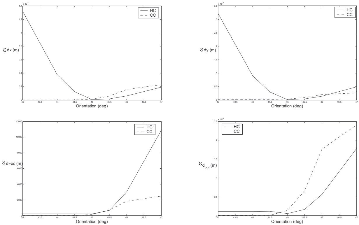
Figure 6 – The square error of the time response \epsilon versus the estimation orientation angle \hat{\theta}_c for the HC and the CC with \delta y_d = 10^{-3} \text{m} .
