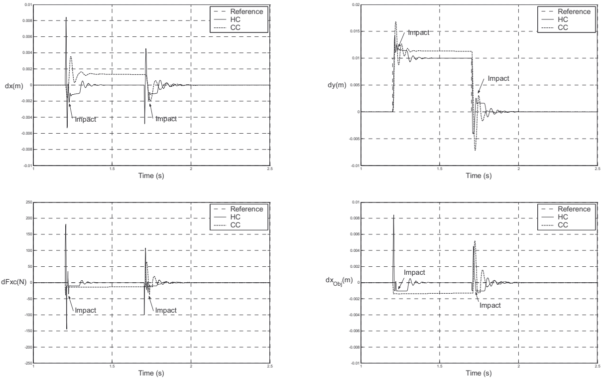
Figure 4 – Time response for the 2R robot under the action of the FO algorithm for the HC and the CC , \delta y_d = 10^{-3} \text{ m} , \hat{\theta}_c = \theta_c = 45^\circ .
