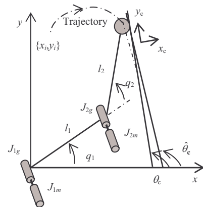
Figure 1 – The 2R robot and the constraint surface.
