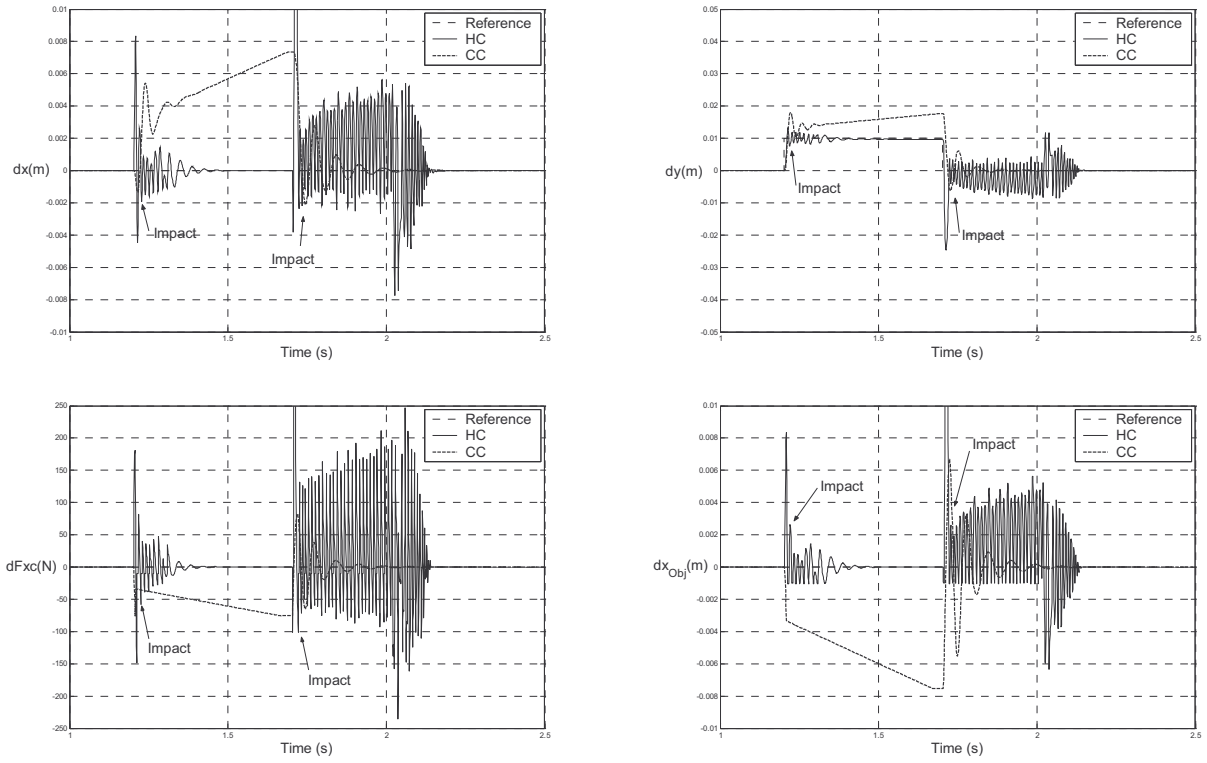
Figure 5 – Time response for the 2R robot under the action of the FO algorithm for the HC and the CC, \delta y_d = 10^{-3} \text{m} , \hat{\theta}_c = 46 degree.
