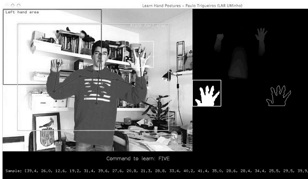
Figure 93. Static gesture feature extraction and model learning user interface
