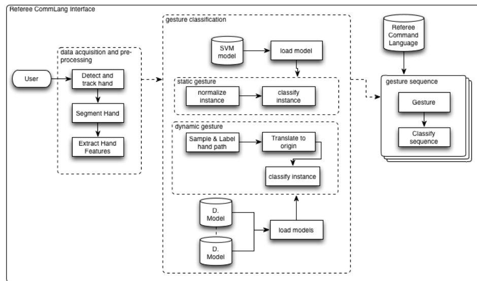
Figure 46. Referee CommLang Interface diagram with all the modules
