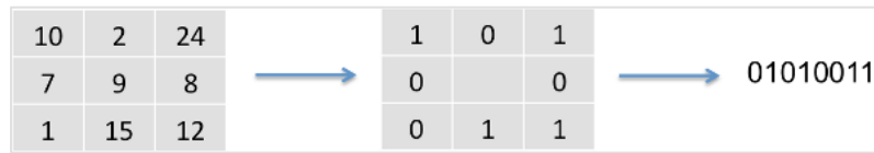
Figure 1. Example of a LBP_{8,1} computation.
