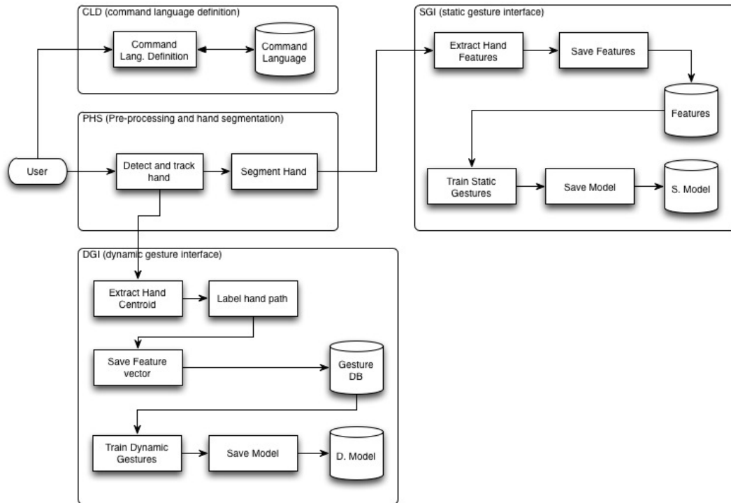
Figure 6. The static and dynamic gesture training and learning architecture.
