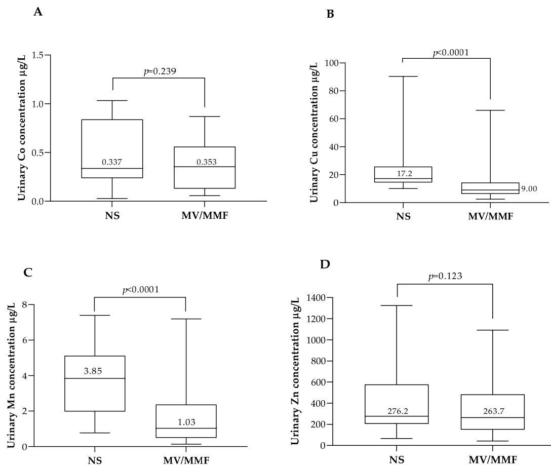
Figure 2. Maternal urinary concentrations of Co (A), Cu (B), Mn (C), and Zn (D) in the 1st trimester according to food supplement use. In each box, the median value (in \mu\text{g/L} ) is indicated above the corresponding central horizontal line. p values (Mann–Whitney) are indicated in each panel. MV/MMF: multivitamin/multimineral formulation users; NS: non-users of supplements.
