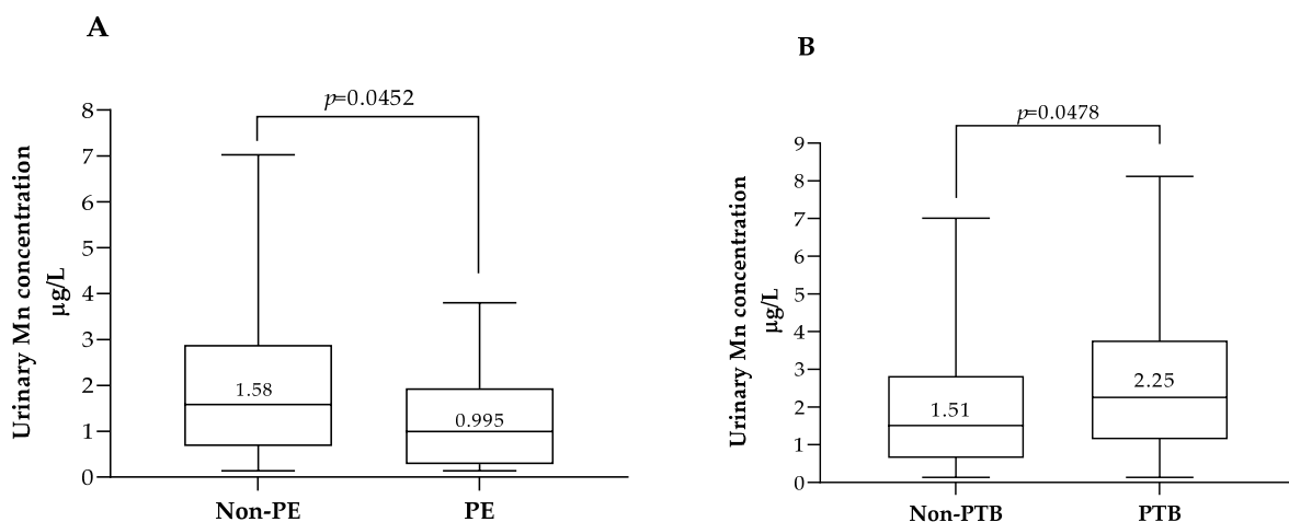
Figure 4. First-trimester maternal urinary Mn concentrations according to the type of pregnancy complication. (A), Mn concentrations in pregnancies with preeclampsia (PE, n = 16 ) or pregnancies without preeclampsia (Non-PE, n = 579 ). (B), Mn concentrations in pregnancies with preterm delivery (PTB, n = 25 ) or non-preterm delivery (Non-PTB, n = 571 ). In each box, the median value (in \mu\text{g/L} ) is indicated above the corresponding central horizontal line. p values (Mann–Whitney) are indicated in each panel.
