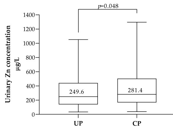
Figure 3. First-trimester maternal urinary Zn concentrations in uncomplicated (UP, n = 476 ) and complicated (CP, n = 120 ) pregnancies. In each box, the median value (in \mu\text{g/L} ) is indicated above the corresponding central horizontal line. p value (Mann–Whitney) are indicated.
