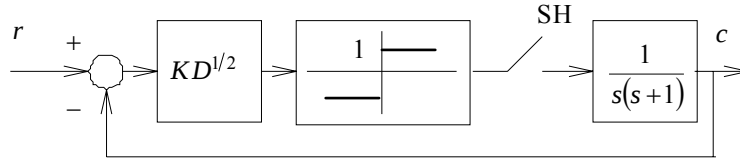
Figure 1. The D^{1/2} controller for a system with a nonlinear actuator.
