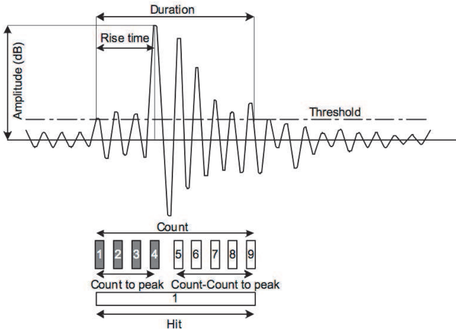
Fig. 2. Conventional AE signal features (Shiotani, 2008)
